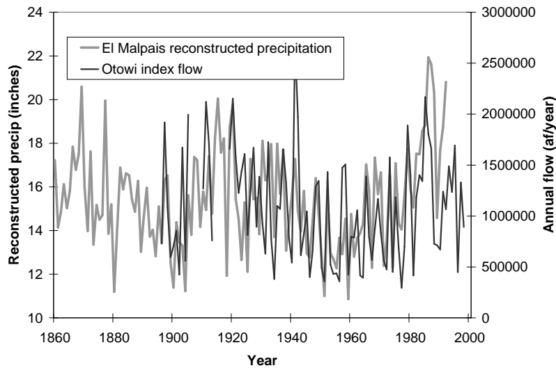
Figure 1: El Malpais reconstructed precipitation versus flow at Otowi Bridge (raw Otowi flow from 1860-1939; Otowi index flow from 1940-1998).
